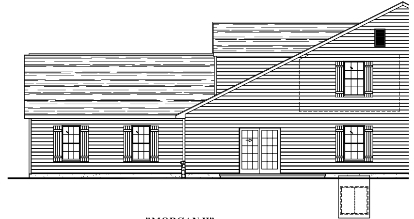
"MORGAN II" SIDE ELEVATION
