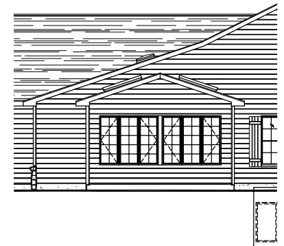
"MORGAN" RANCHER W/ SUNROOM OPTION SIDE ELEVATION
