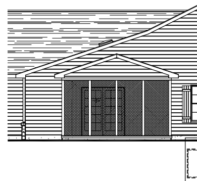
"MORGAN" RANCHER W/ SCREENED-IN PATIO OPTION SIDE ELEVATION
