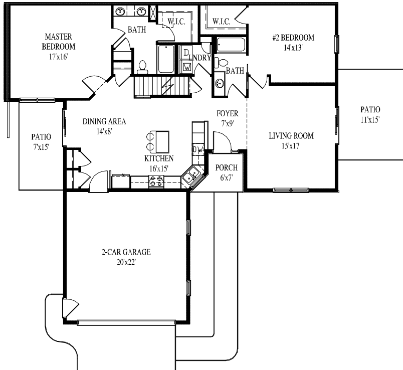
FIRST FLOOR PLAN 1549 SQ. FT.
